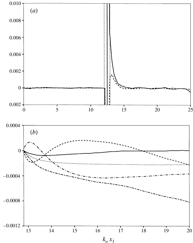
FIGURE 4. (a) Evolution of pressure-dilatation correlation and entropy-dilatation correlation for M_1 = 2.0 : —, \overline{p'u''_{k,k}}/\gamma\bar{p}u_o k_o ; ----, -\overline{s'u''_{k,k}}/c_p u_o k_o . Vertical lines denote the boundaries of shock intermittency. (b) Evolution of the integrated quantities from the acoustic energy balance for M_1 = 2.0 : ----, A; ..... , B; —·—·, C; ———, A + B + C; ———, A + B + C + D.
