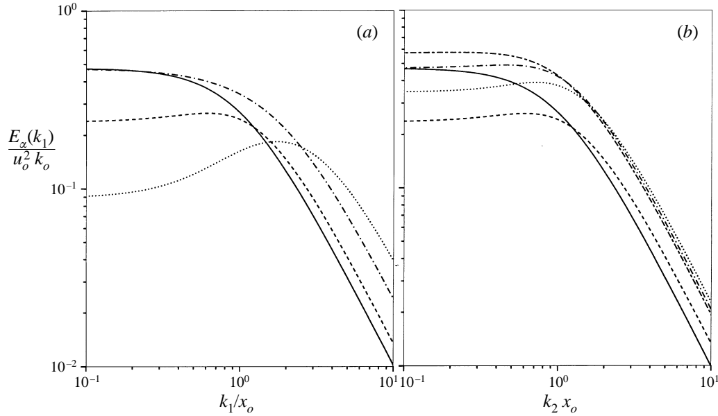
FIGURE 6. LIA prediction of one-dimensional energy spectra changes across the shock wave for (a) M_1 = 2.0 vs. k_1 . E_1 : ———, upstream; — — —, downstream. E_2, E_3 : - - - -, upstream; ·····, downstream. (b) M_1 = 2.0 vs. k_2 . E_2 : ———, upstream; — — —, downstream. E_1 : - - - -, upstream; ·····, downstream; E_3 : - - - -, upstream; — — —, downstream.
