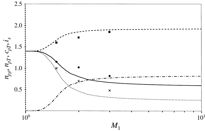
FIGURE 12. Downstream polytropic exponents and entropy fluctuation contribution predicted by LIA. —, n_{\rho\rho} ; - - -, n_{\rho T} ; ·····, c_{\rho T} ; — · —, entropy fluctuation contribution ( i_s ). Symbols for DNS: •, n_{\rho\rho} ; ■, n_{\rho T} ; ×, c_{\rho T} .
