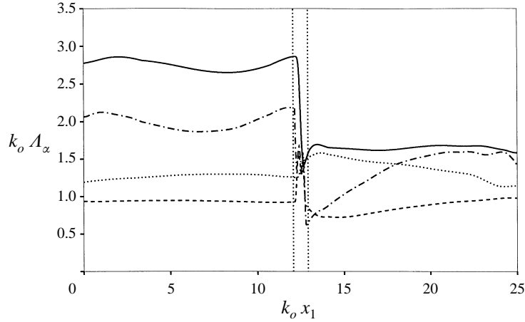
FIGURE 8. Evolution of integral scales throughout the computational domain for M_1 = 2.0 : —, A_{u_2} ; ----, A_{u_1} ; ·····, A_{u_3} ; — · —, A_\rho . Vertical lines denote the boundaries of shock intermittency.
